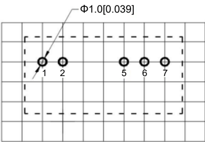
注: 栅格距离尺寸为2.54*2.54mm
